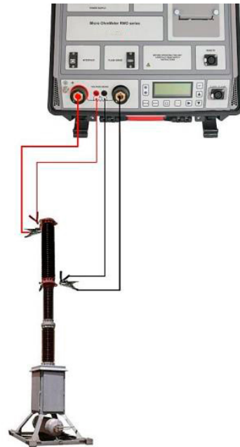
RMO-G cable connection on live tank circuit breaker
