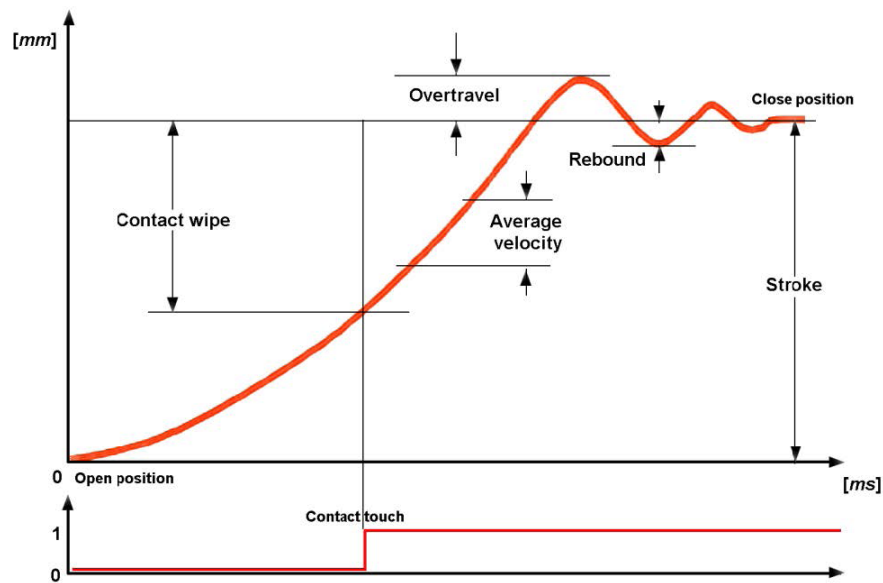
Travel curve and important travel parameters
