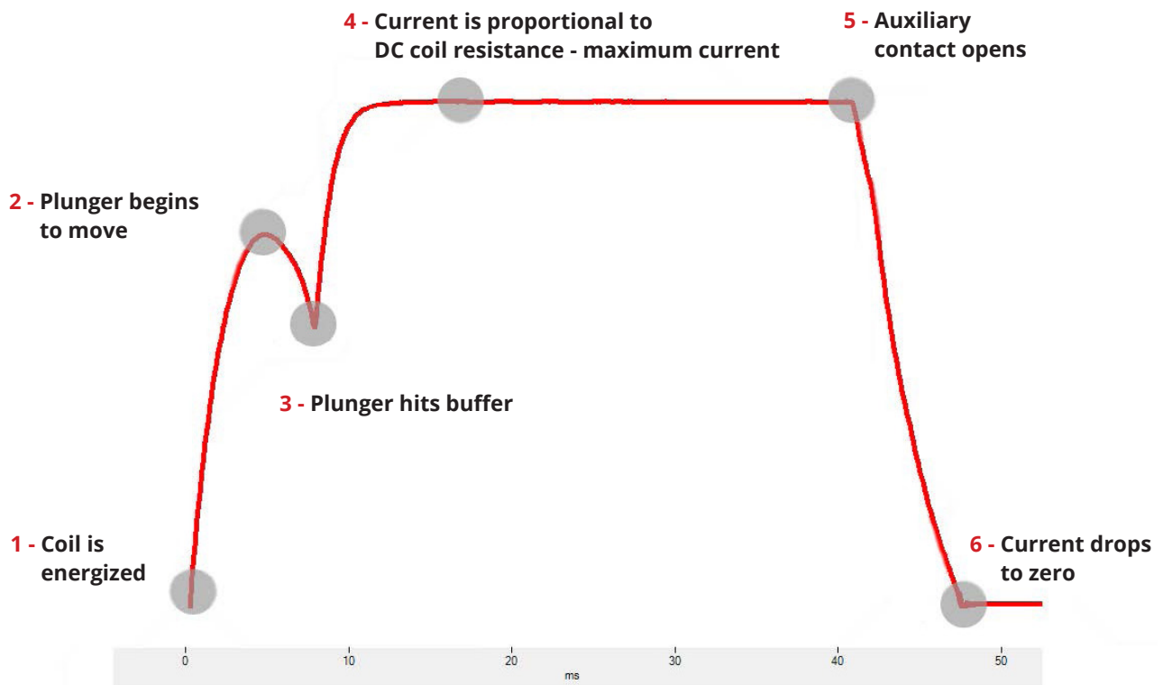
Typical coil current waveform
