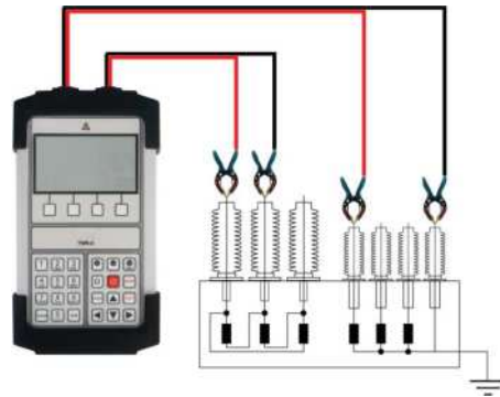
Connecting TWR-H to a three-phase distribution transformer
